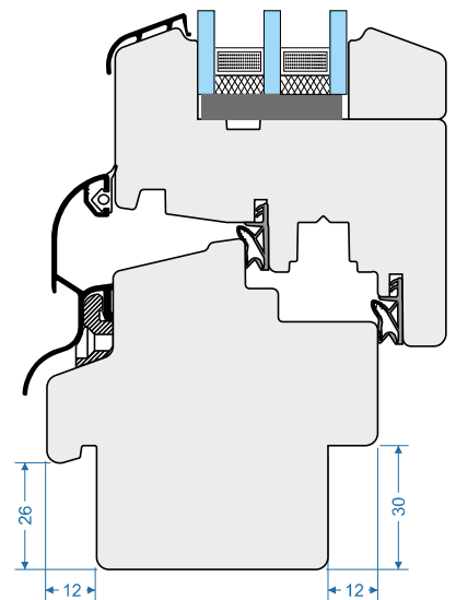
EXT 12x26 INT 12x30
